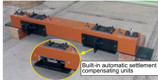
Fig. 1 Automatic settlement compensating sleeper (Type S)
