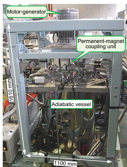
Fig. 1 A small test device to verify the high-temperature superconductive magnetic bearing system
