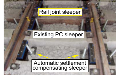
Fig. 2 Automatic settlement compensating sleeper (Type SS)
