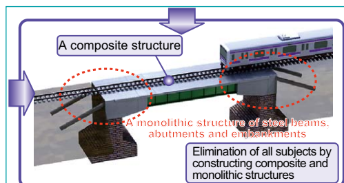
Fig. 4 A combination of composite and monolithic structures
