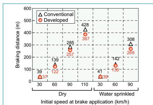
Fig. 3 Results of the performance tests of cars equipped with brake shoes featuring an elastic structure
