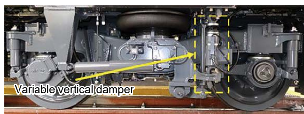
Installation status of a variable vertical damper on an actual vehicle
